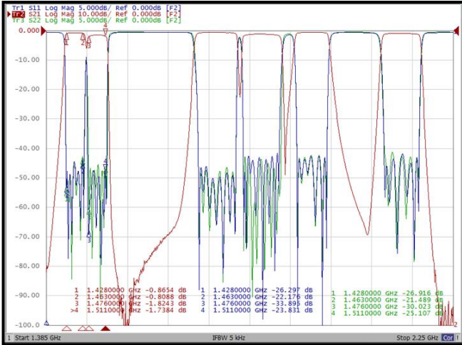
< S21 measurement >
