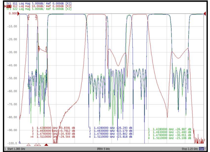
< S12 measurement >
