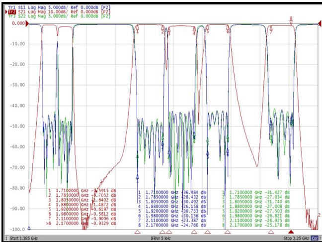
< S21 measurement >
