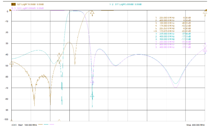
< Insertion Loss / Return Loss measurement >
