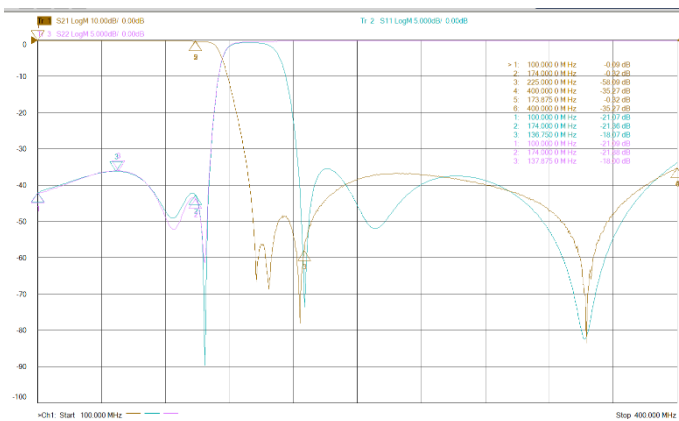
< Insertion Loss / Return Loss measurement >
