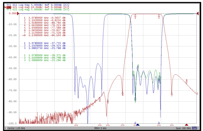
< 1078 ~ 1102MHz measurement >
