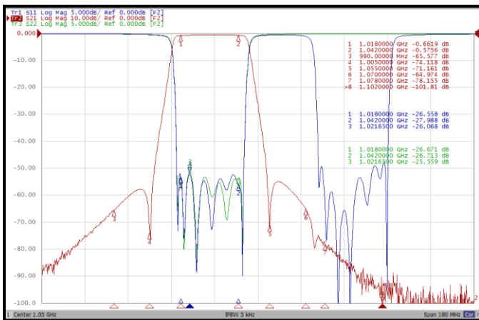
< 1018 ~ 1042MHz measurement >
