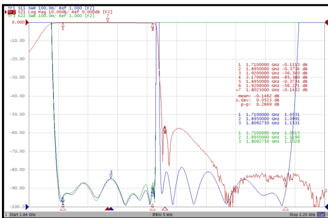
< 1.8GHz measurement >
