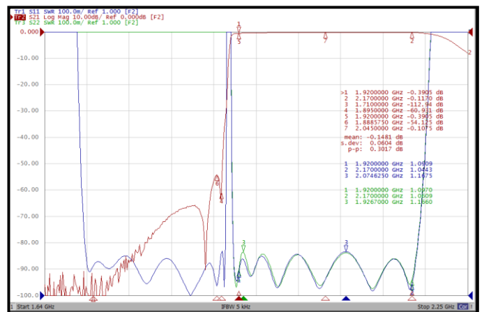
< 2.1GHz measurement >
