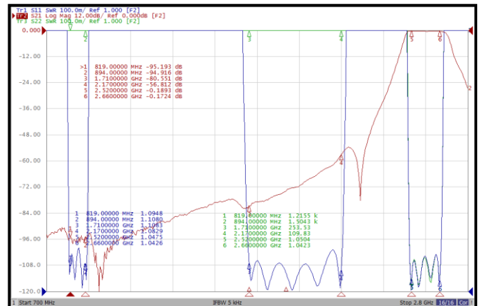
< 2.6GHz Isolation measurement >
